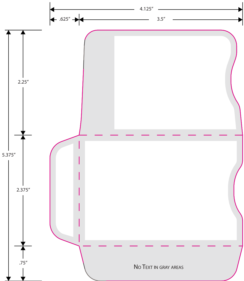
2.375" x 3.5" CCLSH 07/2012 Credit Card L-Seam 2 Card Holder
